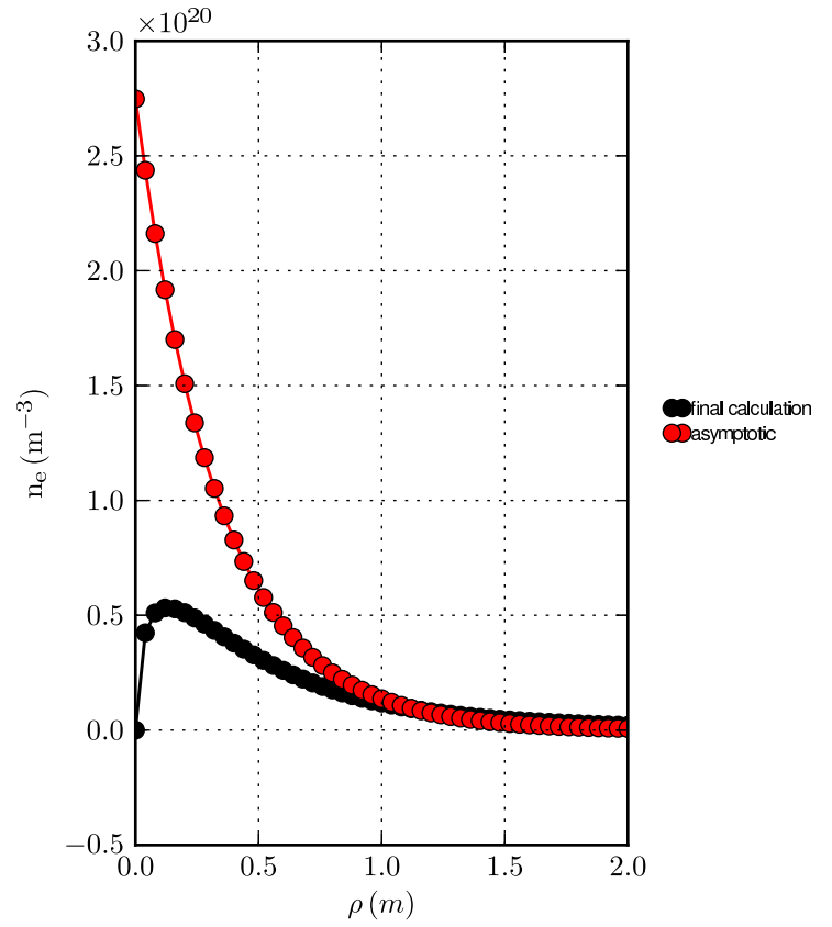
Electron density
