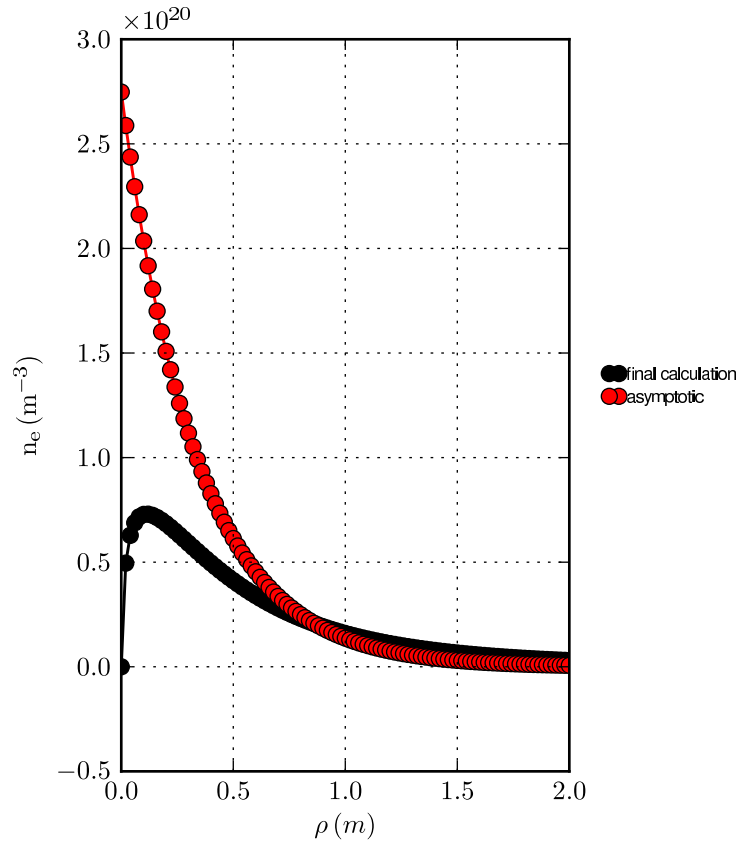
Electron density
