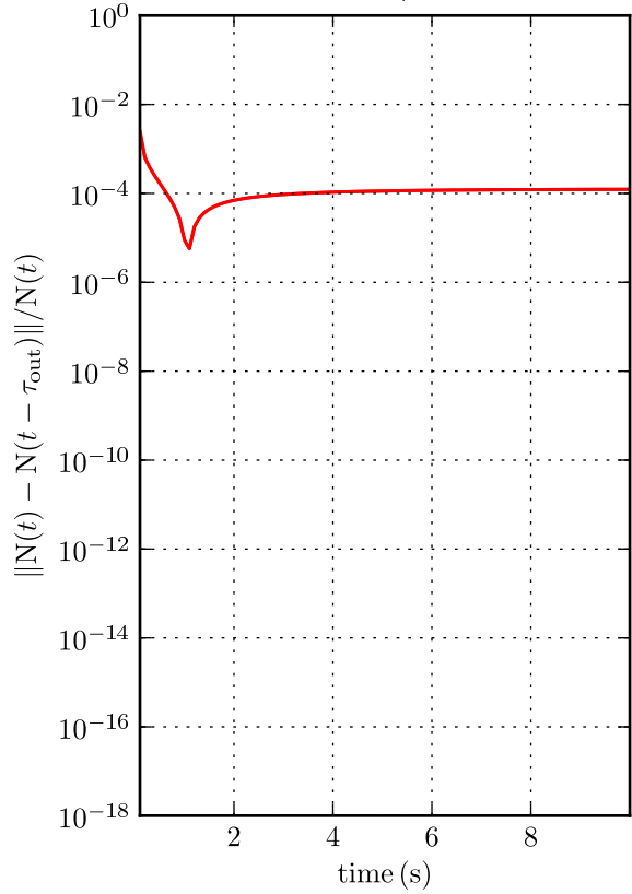
Particle conservation (electrons and ions)
