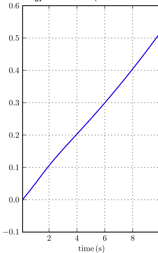
Energy conservation (electrons and ions)
